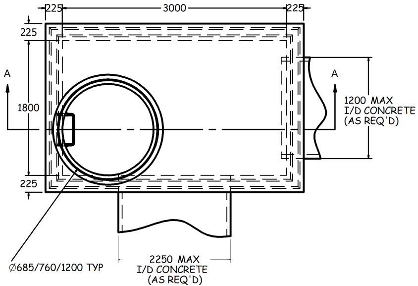
TOP VIEW 1:50
