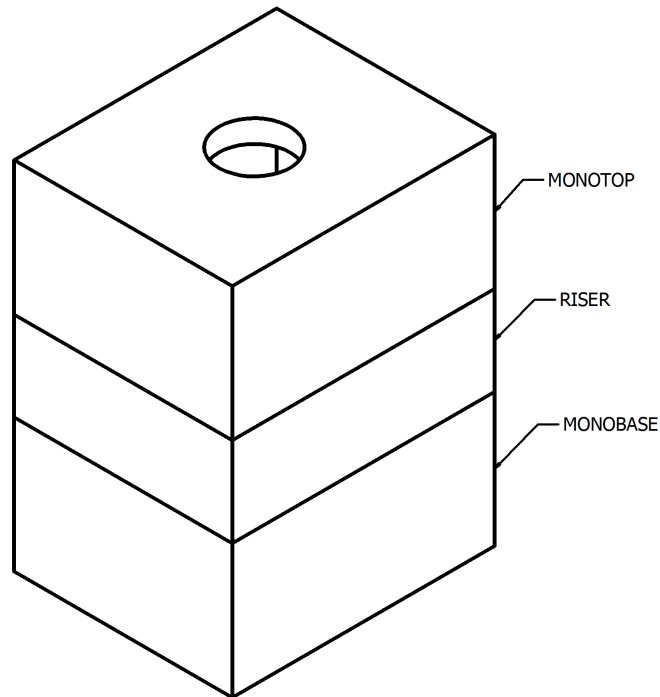
ISOMETRIC VIEW 1:60
