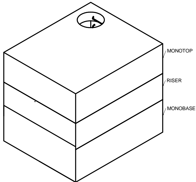
ISOMETRIC VIEW 1:55
