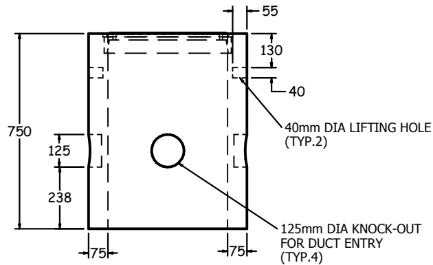
FRONT VIEW 1:20
