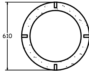
SECTION VIEW 1:20
