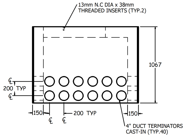
FRONT VIEW 1:30
