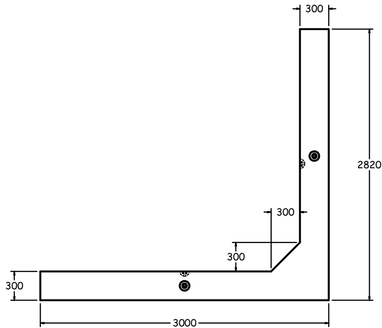
WINGWALL "L" COMPONENT
