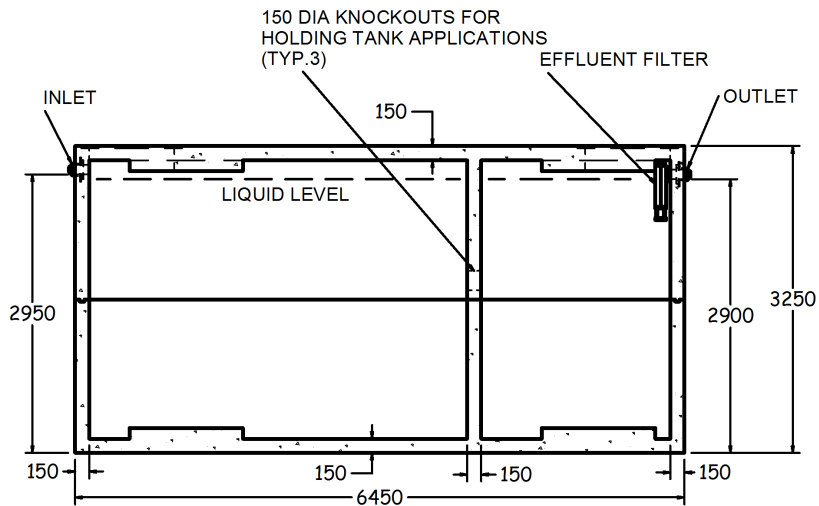
SIDE SECTION 1:80
