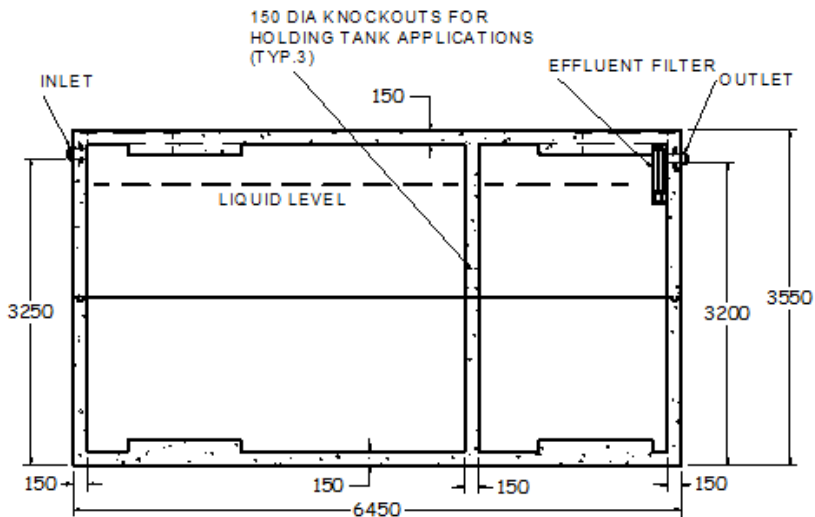
SIDE SECTION 1:80
