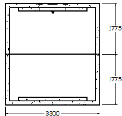
END SECTION 1:80
