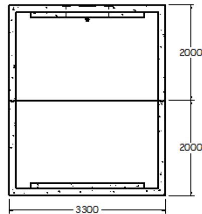
END SECTION 1:80
