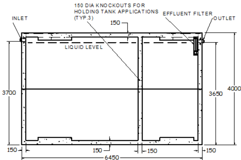
SIDE SECTION 1:80
