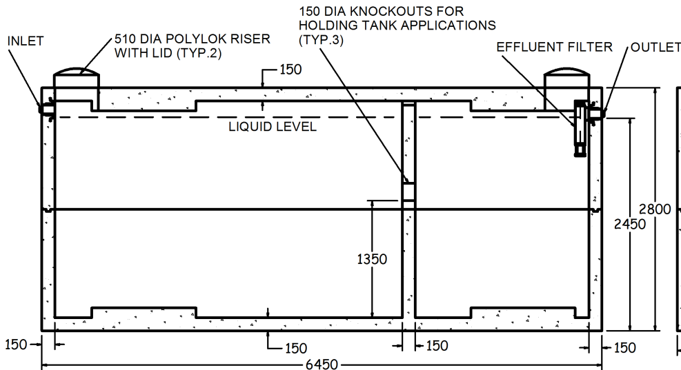
SIDE SECTION 1:60
