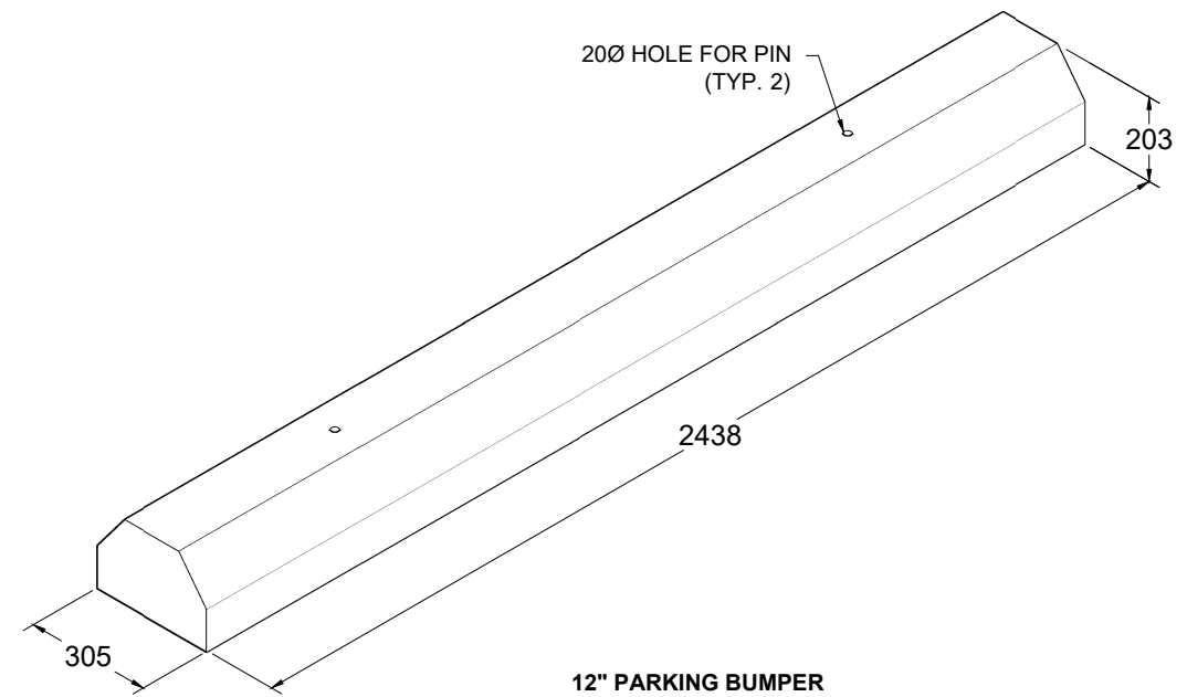
12" PARKING BUMPER 305 x 2438 x 203 (12" x 96" x 8") 317kg ea.
