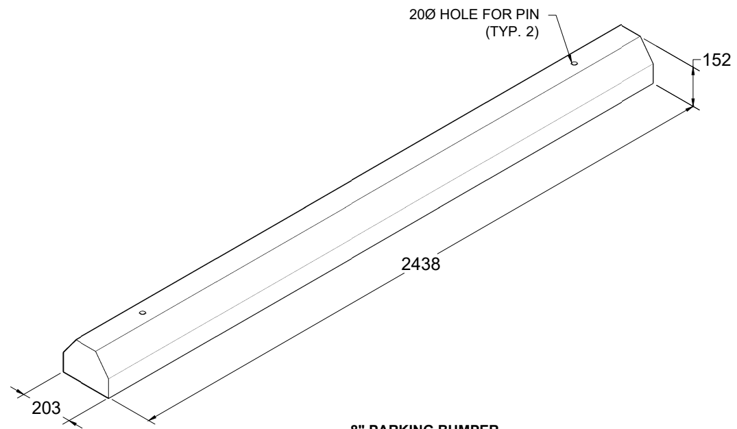
8" PARKING BUMPER 203 x 2438 x 152 (8" x 96" x 6") 155kg ea.
