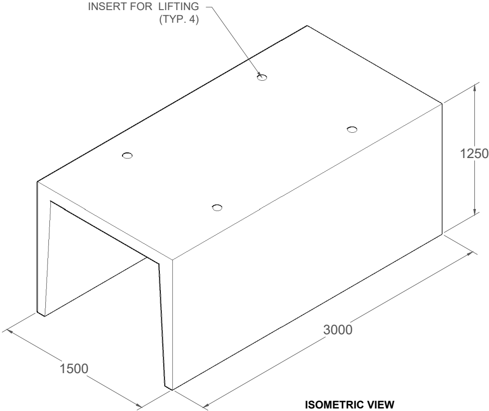
ISOMETRIC VIEW TROUGH 3000mm x 1500mm x 1250mm 3050 KG
