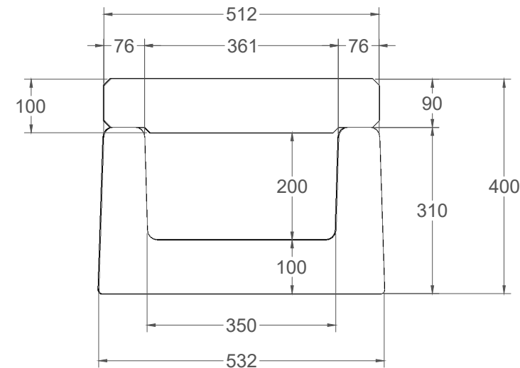
SECTION VIEW
