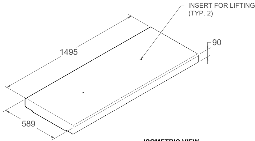
ISOMETRIC VIEW LID 1495mm x 589mm x 90mm 210 KG
