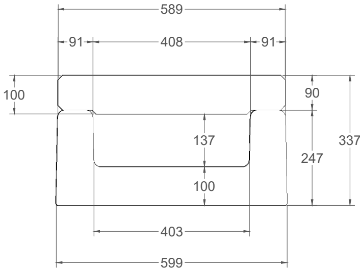
SECTION VIEW
