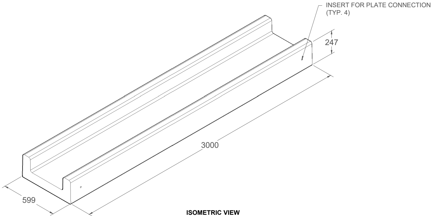
ISOMETRIC VIEW TROUGH 3000mm x 599mm x 247mm 630 KG
