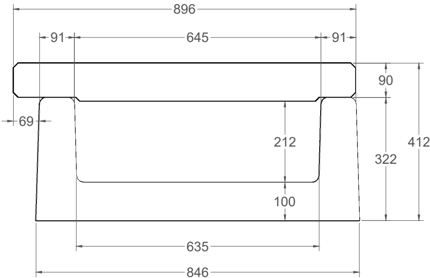
SECTION VIEW
