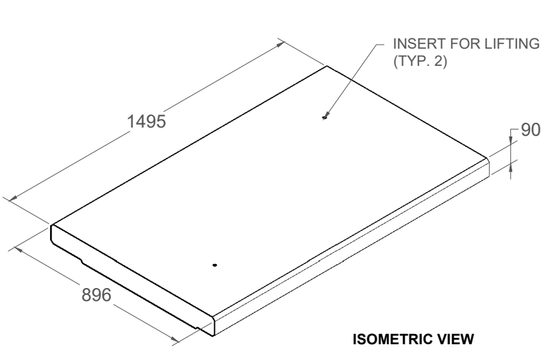
ISOMETRIC VIEW LID 1495mm x 896mm x 90mm 315 KG
