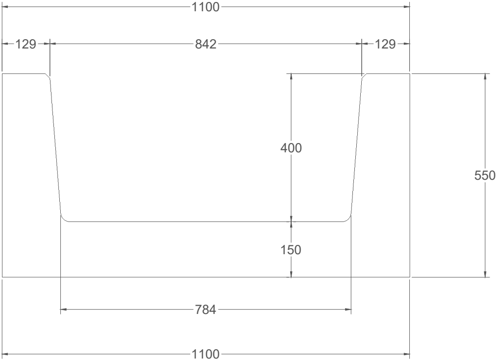
SECTION VIEW
