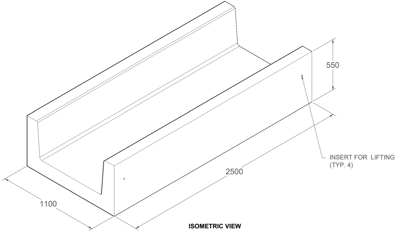
ISOMETRIC VIEW TROUGH 2500mm x 1100mm x 550mm 1690 KG
